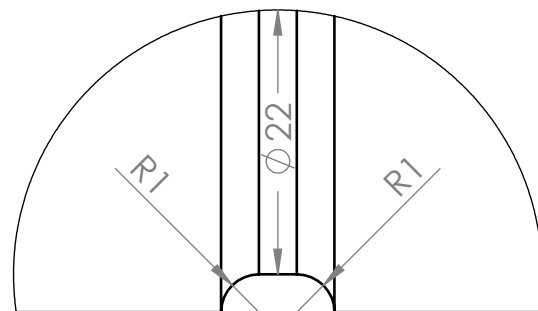
DETAIL B SCALE 5 : 1
